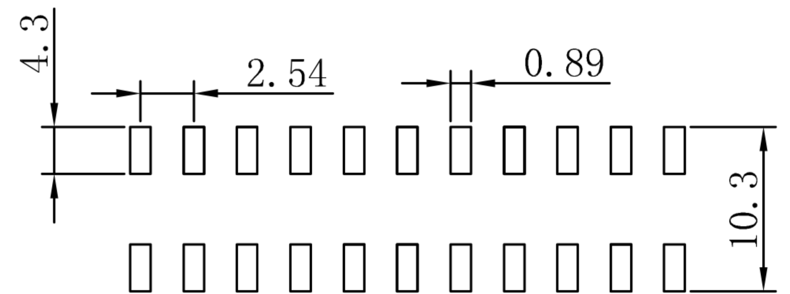
PCB LAYOUT
