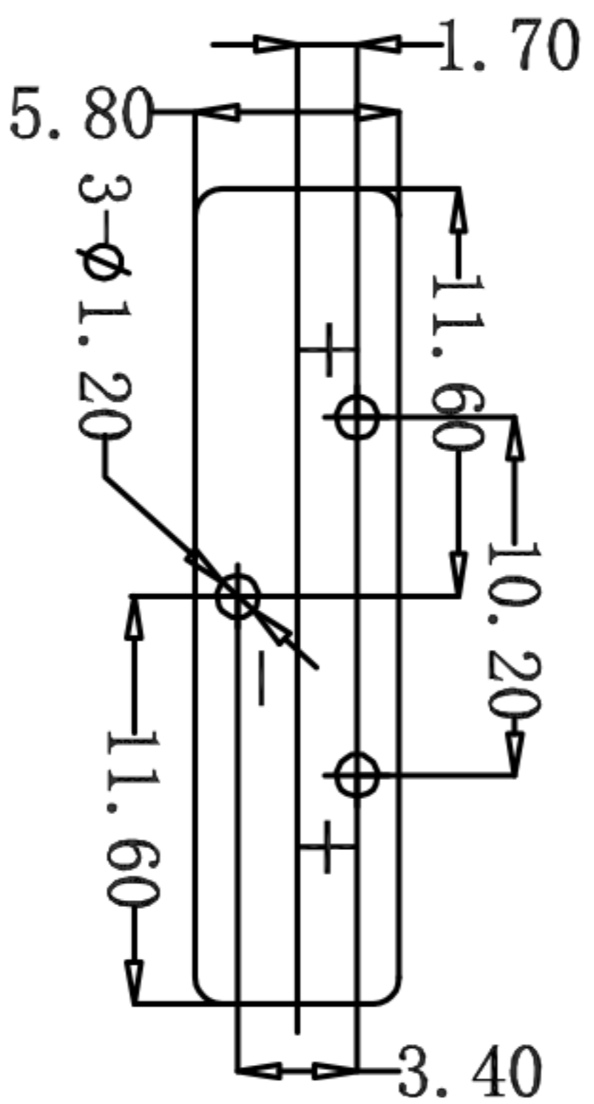
PCB Layout Diagram Top View
