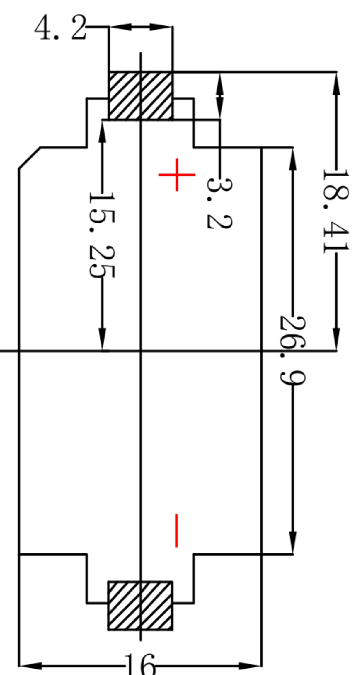
PCB Layout Diagram Top View
